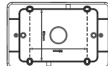
A3223HSME Rear View
